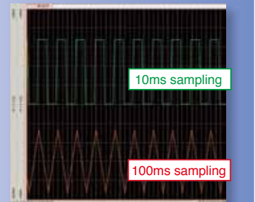
Measurement comparison of 5 Hz square pulse waveform with 10 ms (upper trace) and 100 ms sampling
